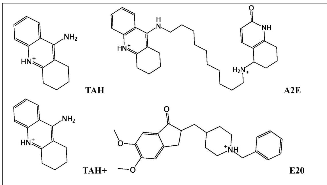
Figure 1: Structures of neutral tacrine (TAH, top left), positively charged tacrine (TAH+, bottom left), tacrine-hupyradone inhibitor (A2E, top right) and aricept (E20, bottom right)
