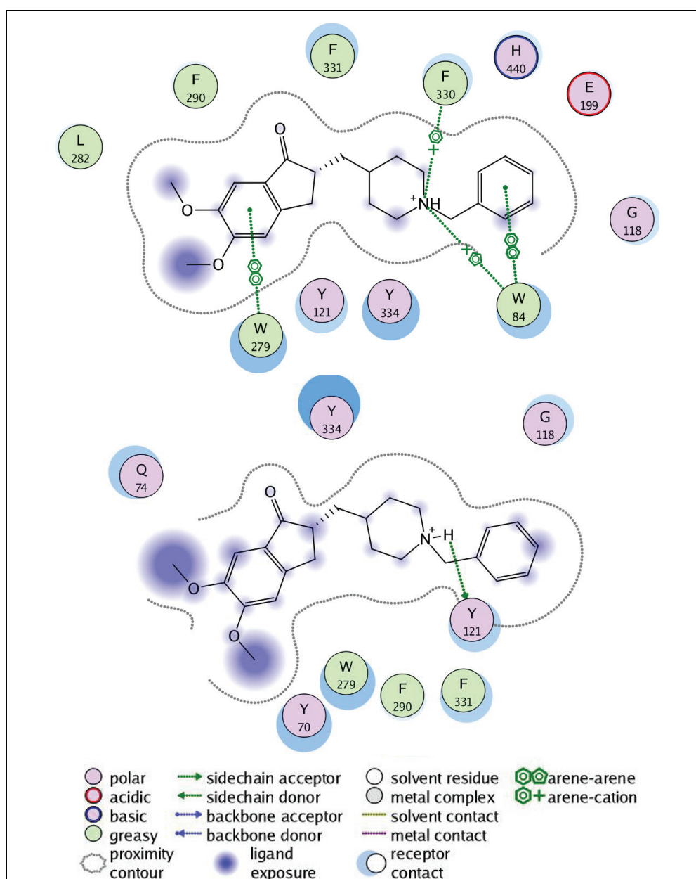
Figure 3: Experimental (1eve PDB file, top panel) and predicted (FlexX re-docking, bottom panel) binding mode between E20 and acetylcholinesterase. The pictures were prepared using MOEv2009.10.
